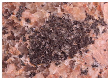
Fig. 5. Ross of Mull Granite at Locality 3 with xenoliths of meta-sedimentary rock.
